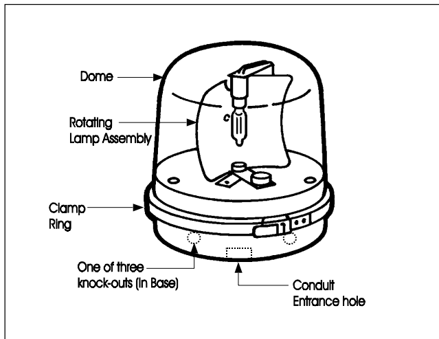
Figure 1. Catalog Series 58-N5-100WH Signal
