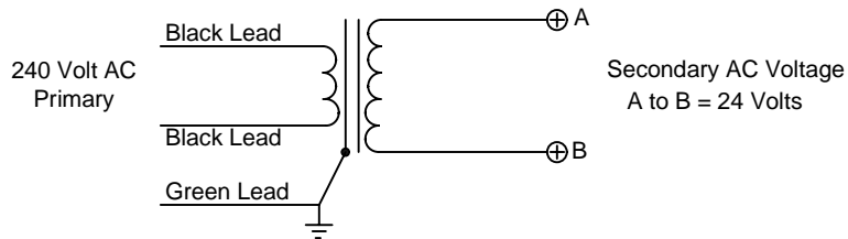
599Y Transformer
