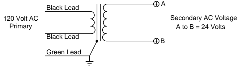
599 Transformer
