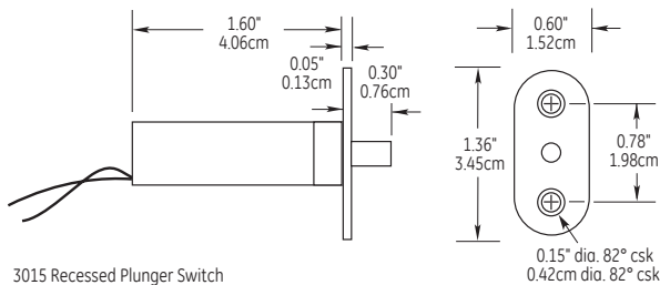
3015 Recessed Plunger Switch Includes: 1- Adjustable #6 x 32 1/2" Phillips screw
