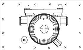
Horizontal Mount
